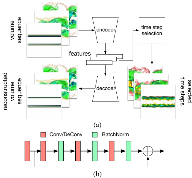
Figure 1: (a) Our approach learns a feature descriptor for each time step (single or multiple variables) and selects representatives in the projected space. We use downsampled volumes as input due to the GPU memory limitation. (b) The diagram of a learning block.
