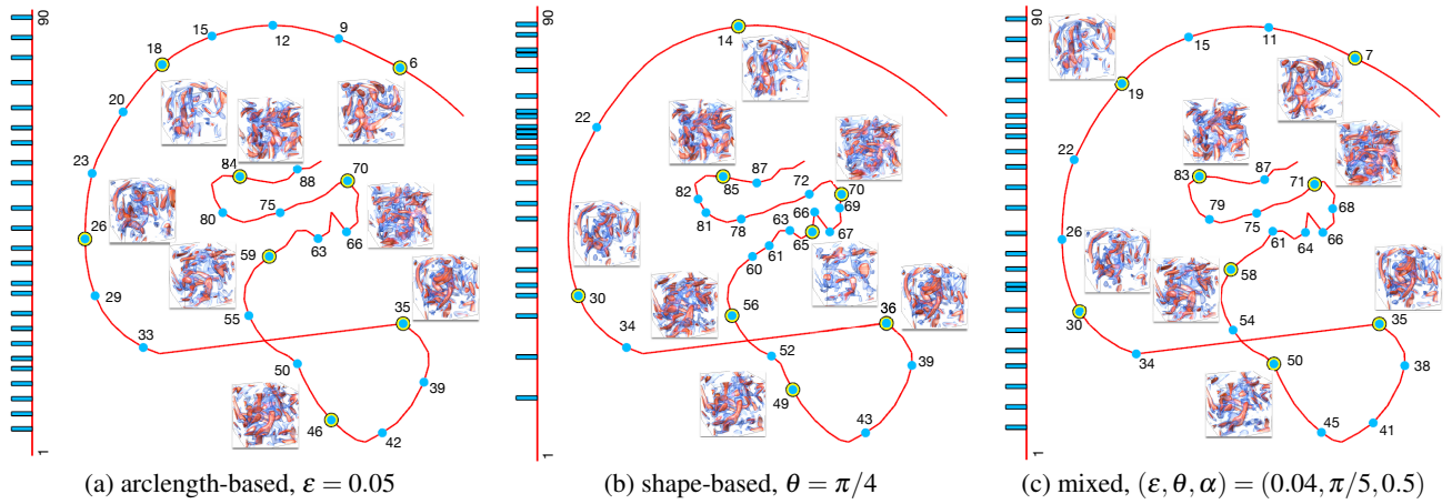
Figure 2: Comparing different ways of time step selection using the vortex data set. All select 24 time steps from 90 time steps. In the t-SNE projection, selected time steps are marked with blue dots and labeled with time step IDs, and those shown along with thumbnails are highlighted. We also indicate selected time steps along the linear vertical timeline.
