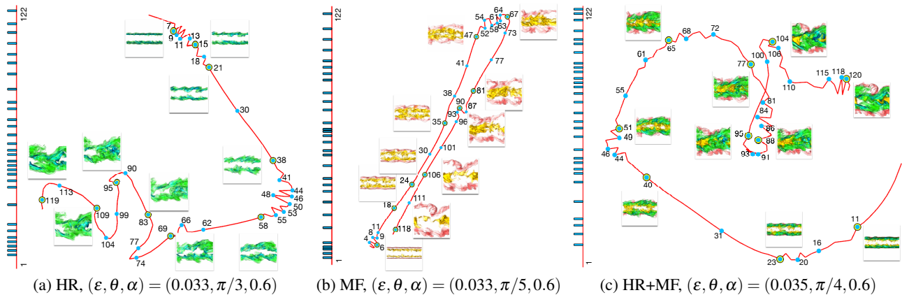
Figure 4: Comparing t-SNE projection and time step selection results under single and multiple variables using the combustion data set. All select 30 time steps from 122 time steps.
