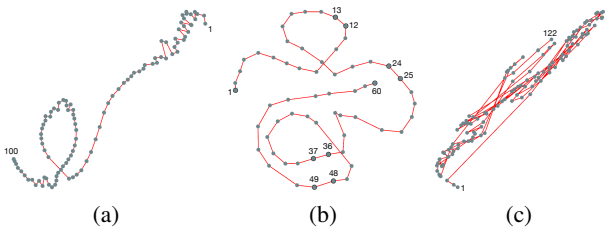
Figure 5: Comparing t-SNE projections using different types of time-varying data sets. (a) ionization, (b) climate, and (c) combustion (CHI). (a) to (c) are for regular, periodic, and turbulent types of data, respectively. Time steps are marked with black dots. In (b), both ends of the periods are highlighted (each period consists of 12 time steps).
